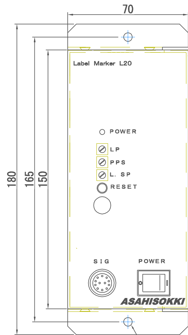
Front view
