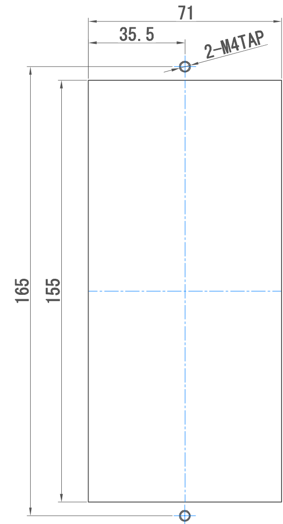
Drilling dimension diagram
